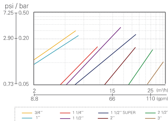
Y TYPE FILTER HEAD LOSS(130 micron/120mesh)
